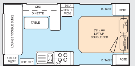
No. 35 (17x7.8) bunk
