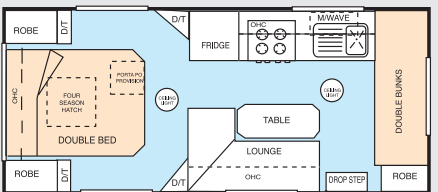
No. 36 (17x7.8) bunk - tunnel boot
