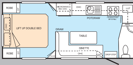
No. 25 (19x7.8) st
