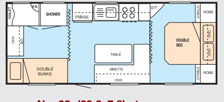
No. 33 (23.6x7.8) st
