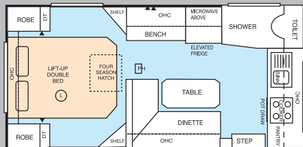
No. 22 (18.6x7.8) st
