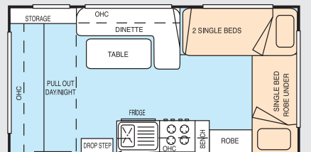
No. 34 (17x7.8) bunk
